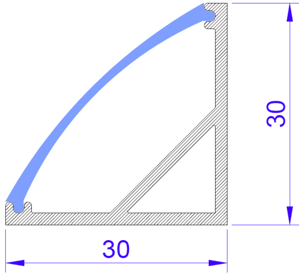
ALD-16 Lengths - 1m, 2m Diffuser - Opal or Translucent
